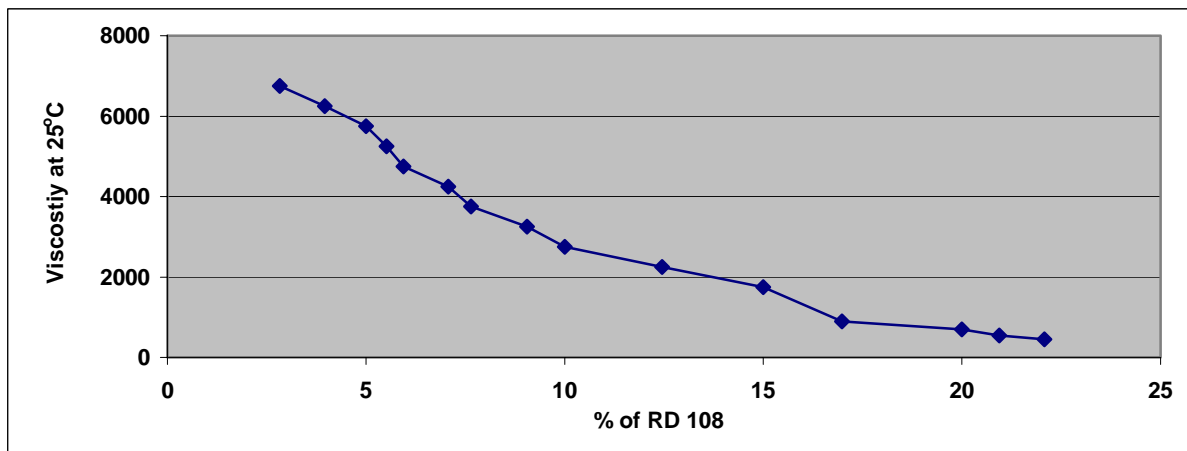
Figure 1 Effect of % of RD 108 on viscosity of standard epoxy resin
