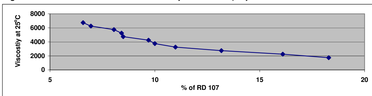
Figure 1 Effect of % of RD 107 on viscosity of standard epoxy resin
